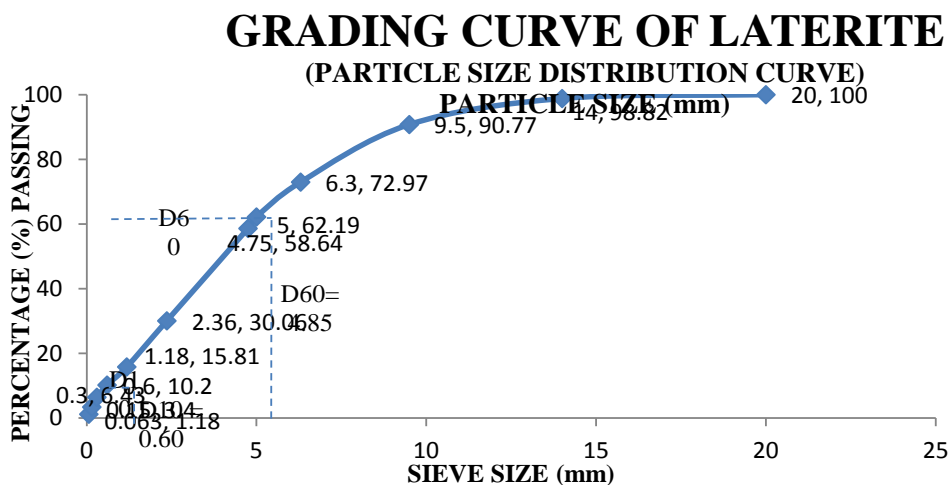
Figure 1 Grading Curve of Laterite (Source: Field Survey, 2011)
