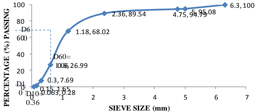
Figure 2 Grading Curve of Sand (Source: Field Survey, 2011)
